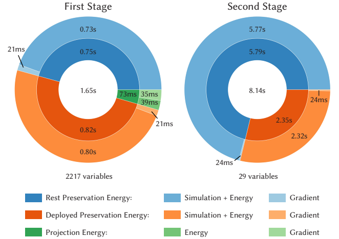
Fig. 17. Timings of our two-stage optimization, reported per each successful line search step as measured on a Linux workstation with a 64-Core AMD Ryzen Threadripper 3990X Processor and 128GB of RAM. The simulation time consists of solving the equilibrium problem possibly multiple times during the linesearch phase of the optimization. Gradient computation relies on the simulation output and is done once per step. For this experiment, the first stage took 1019 steps, and the second stage took 42 steps.
