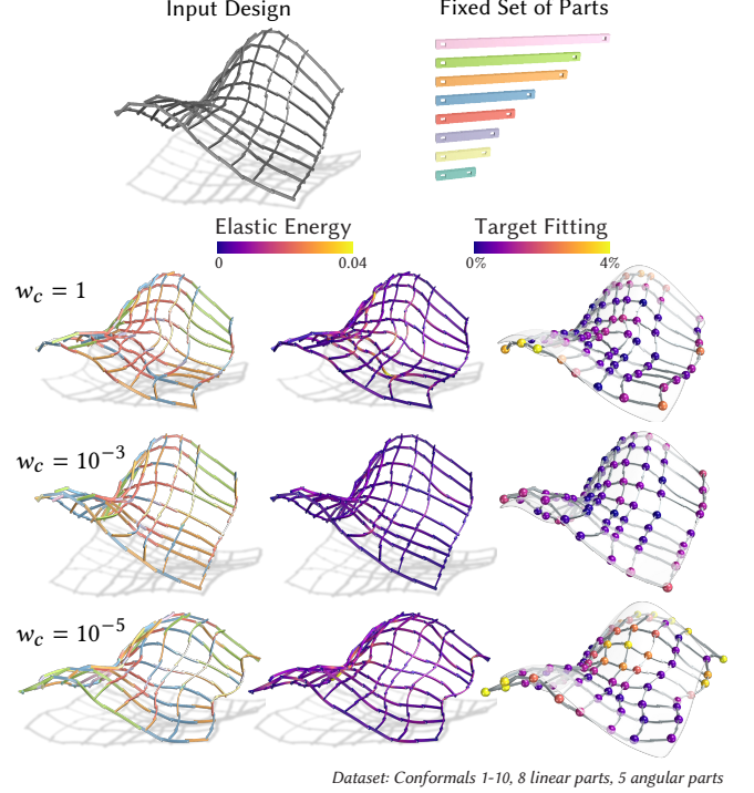
Fig. 13. A new design is projected onto an existing kit of parts. The input design has not been used during the optimization of the kit of parts. Tuning the clustering weight allows recovering a better design.
